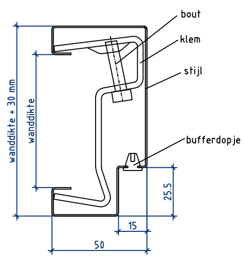
Detail 2: klem
